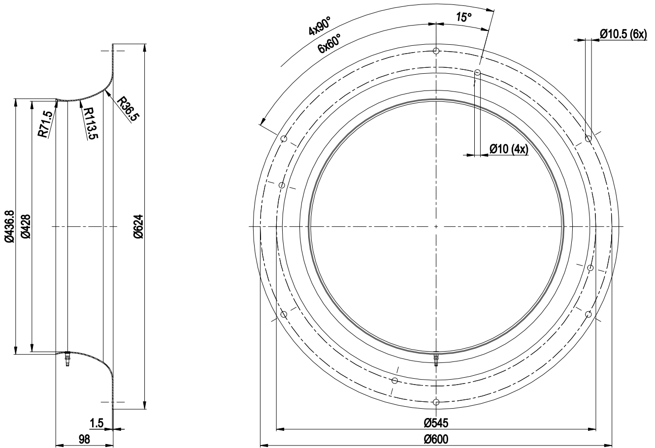
Inlet ring 64045-2-4013 with pressure tap (k-factor: 438)
